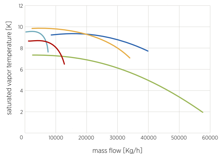
FIMA VARECO performance range for 60 °C.
